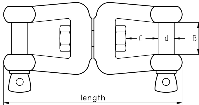
Figure 1: Swivel Shackle with Forks
